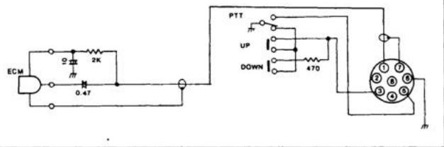
Schematic diagram of IC-SM6
