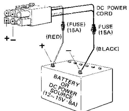
For DC operation
