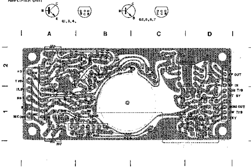
AMPLIFIER UNIT
